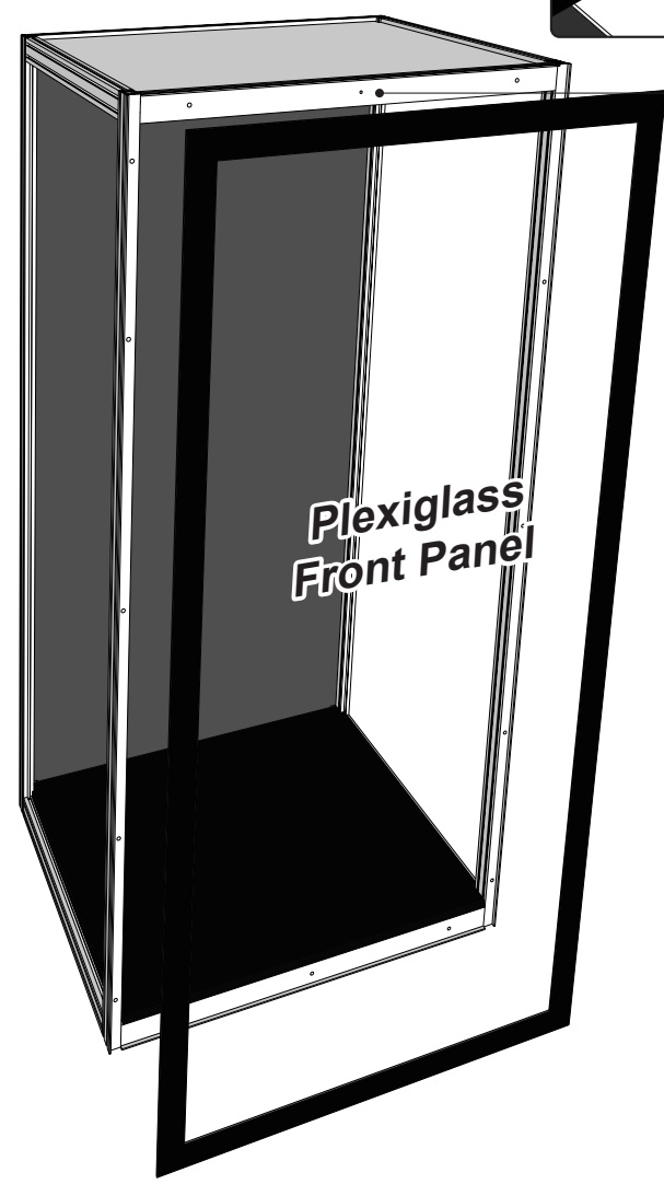
Step 17. Attach the Plexiglass Front Panel and insert the Safety Screw.
